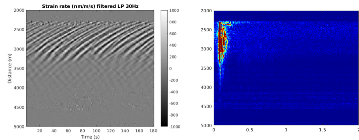
Figure 5: Strain rate recorded at the entrance of the fibre in the water (2.25km) filtered with a low-pass filter at 30Hz. The shallow water ends after around 4.5km of cable. Right: Frequency content of strain rate signal along the fibre
