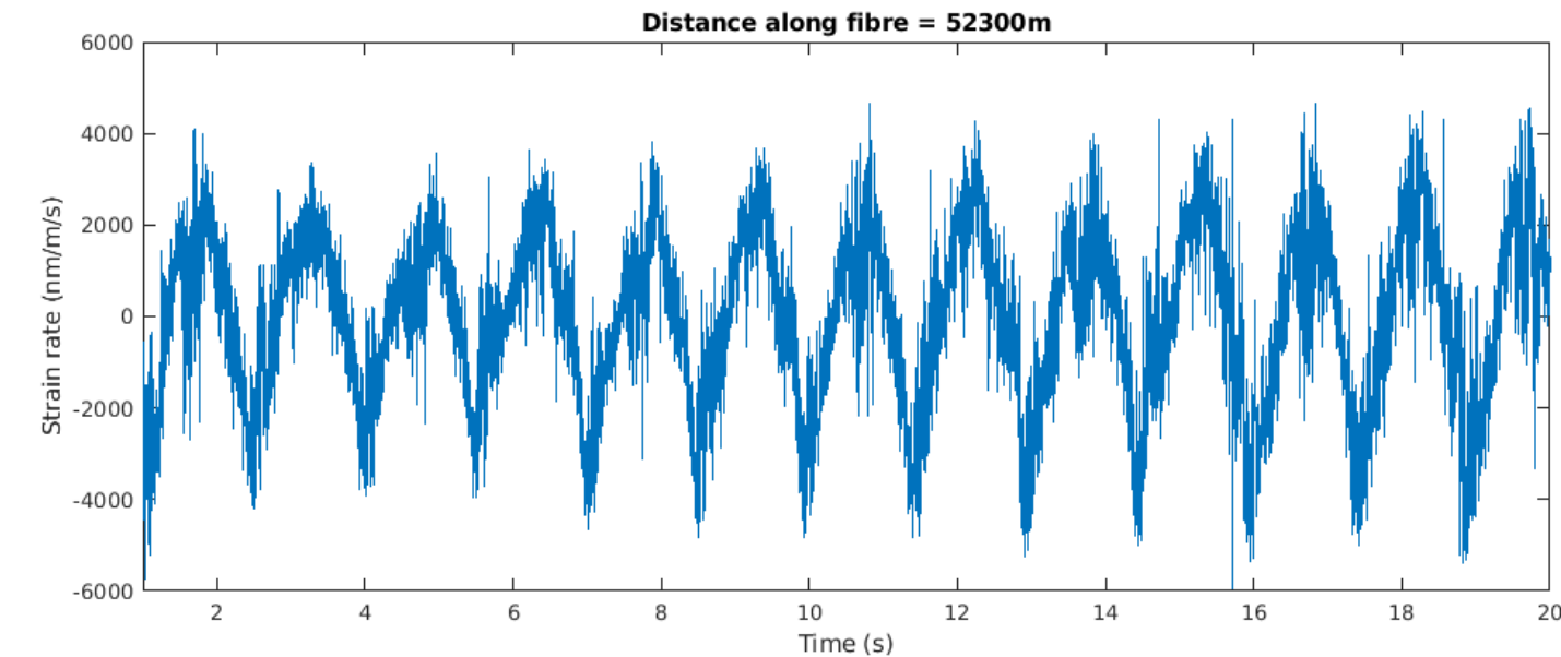
Figure 6: Top left: Strain rate along the end of the fibre (from 50km to 56.5km) filtered with a low-pass filter at 30Hz. Top right: Frequency content of strain rate signal at the same distance. Bottom: Strain rate signal at 52,300m in nm/m/s
