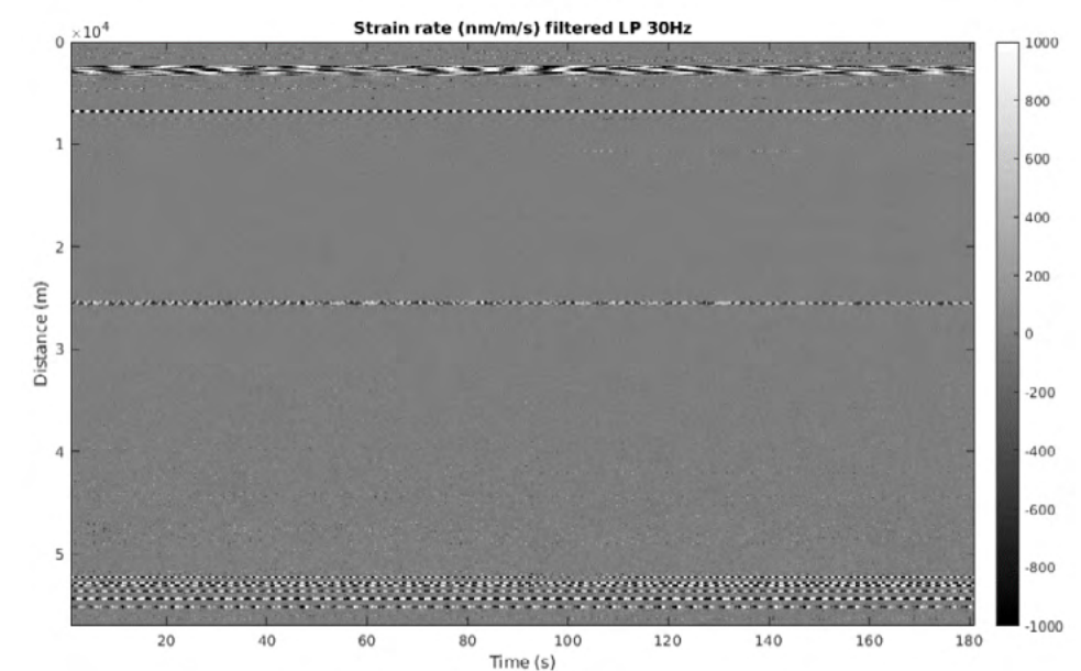
Figure 4: Results of 3 minutes DAS acquisition along the 56.5km-fibre deployed offshore Funchal, Madeira. DAS data are expressed in nm/m/s and are here filtered with a low-pass filter at 30Hz
